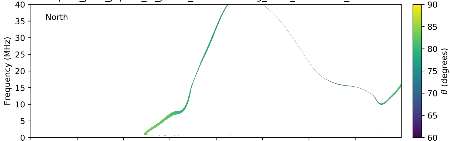
expres_juno_jupiter_io_jrm09_lossc-wid1deg_3kev_20160914_v01.cdf
