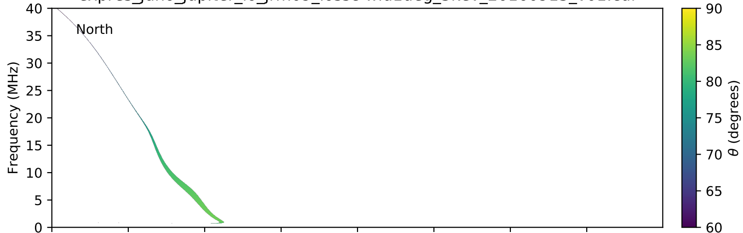
expres_juno_jupiter_io_jrm09_lossc-wid1deg_3kev_20160913_v01.cdf
