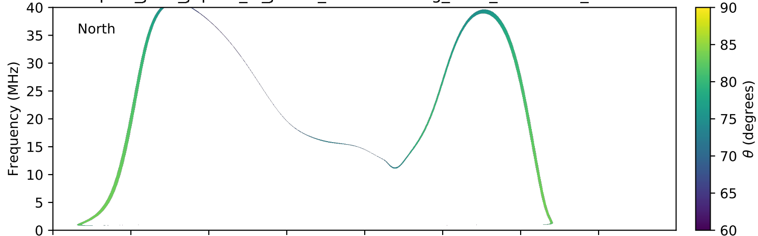
expres_juno_jupiter_io_jrm09_lossc-wid1deg_3kev_20160909_v01.cdf
