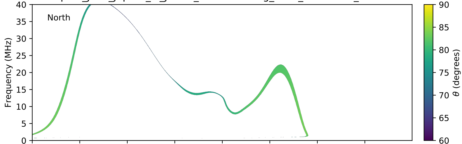
expres_juno_jupiter_io_jrm09_lossc-wid1deg_3kev_20160902_v01.cdf
