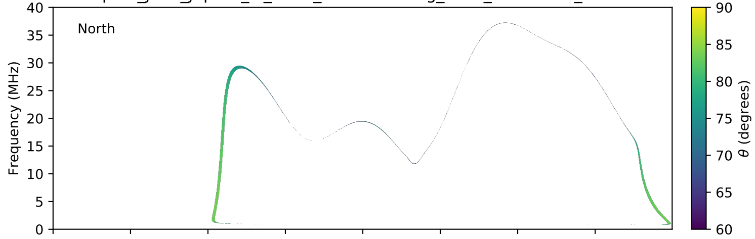
expres_juno_jupiter_io_isaac_lossc-wid1deg_3kev_20160930_v01.cdf
