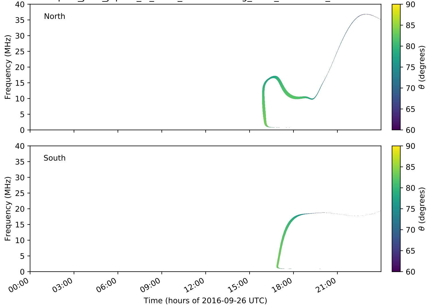
expres_juno_jupiter_io_isaac_lossc-wid1deg_3kev_20160926_v01.cdf
