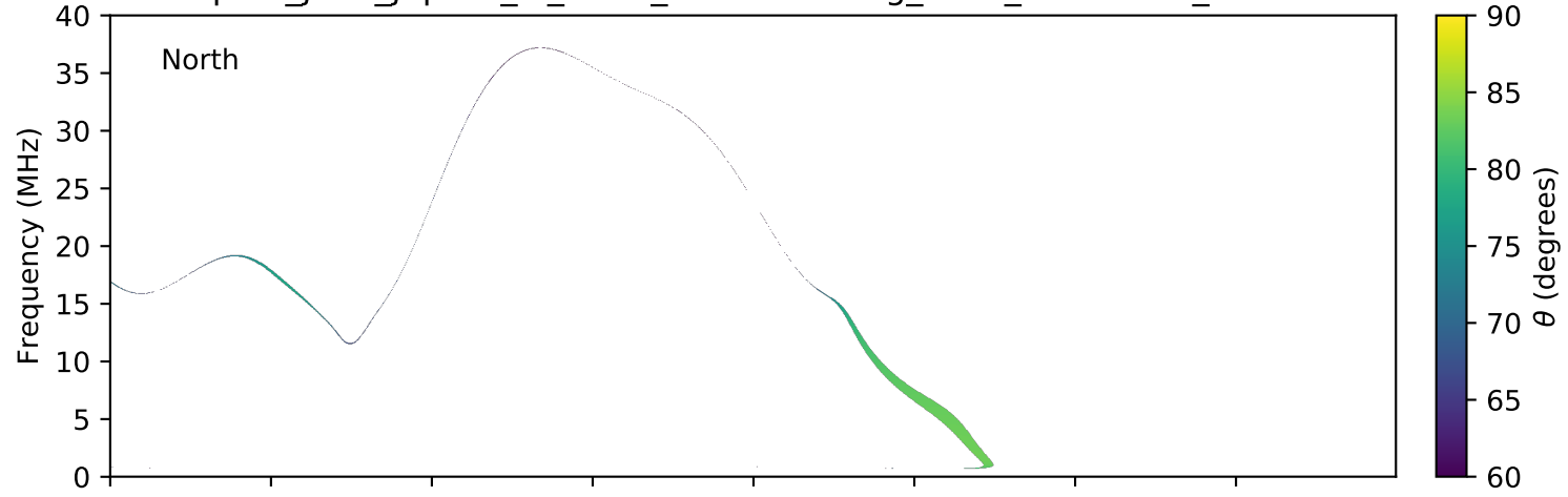
expres_juno_jupiter_io_isaac_lossc-wid1deg_3kev_20160925_v01.cdf
