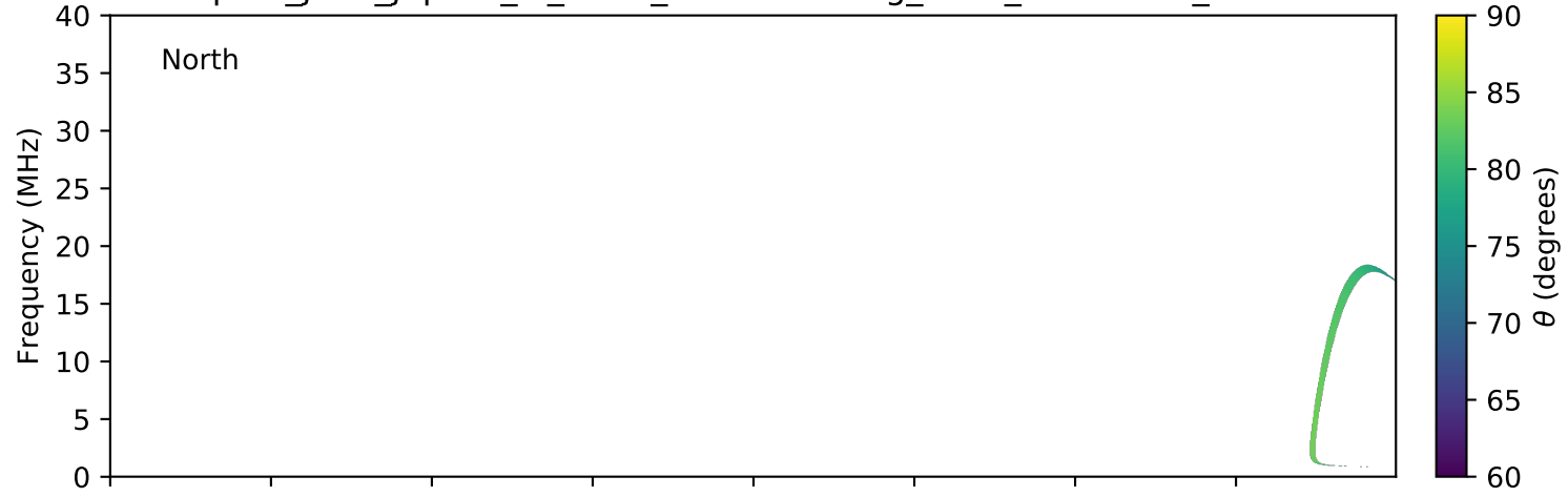
expres_juno_jupiter_io_isaac_lossc-wid1deg_3kev_20160924_v01.cdf
