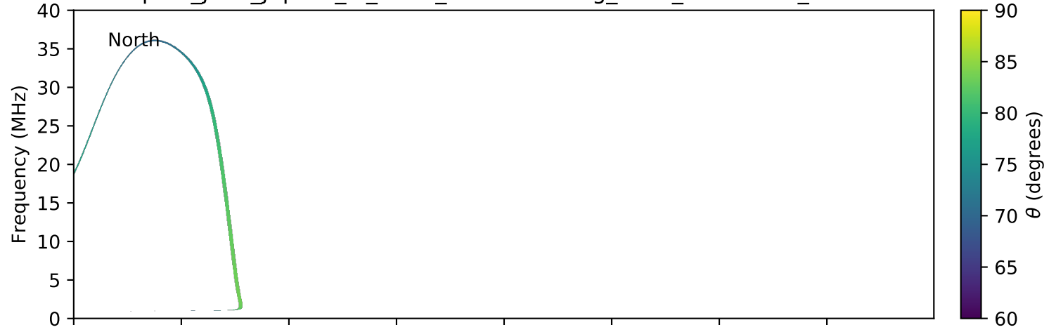
expres_juno_jupiter_io_isaac_lossc-wid1deg_3kev_20160922_v01.cdf
