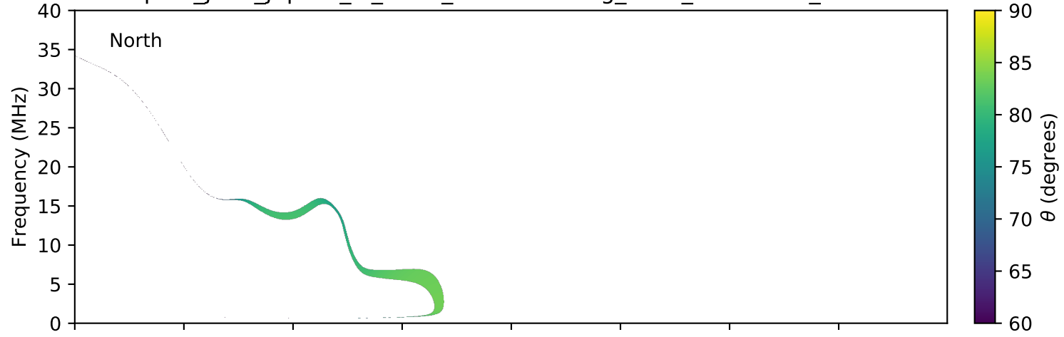
expres_juno_jupiter_io_isaac_lossc-wid1deg_3kev_20160920_v01.cdf
