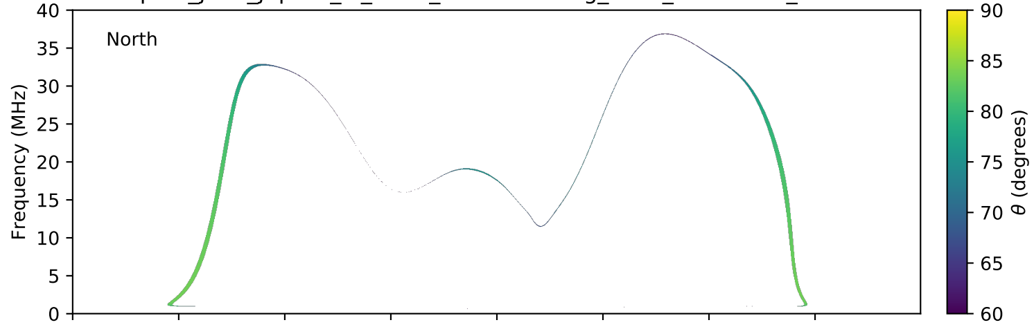
expres_juno_jupiter_io_isaac_lossc-wid1deg_3kev_20160916_v01.cdf
