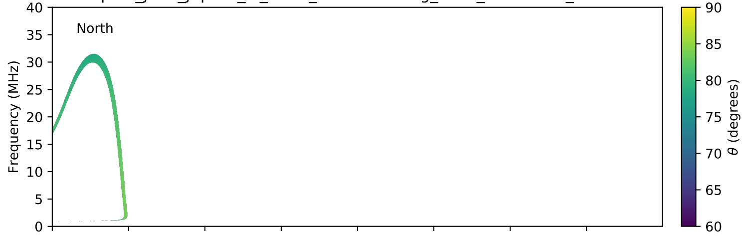
expres_juno_jupiter_io_isaac_lossc-wid1deg_3kev_20160915_v01.cdf
