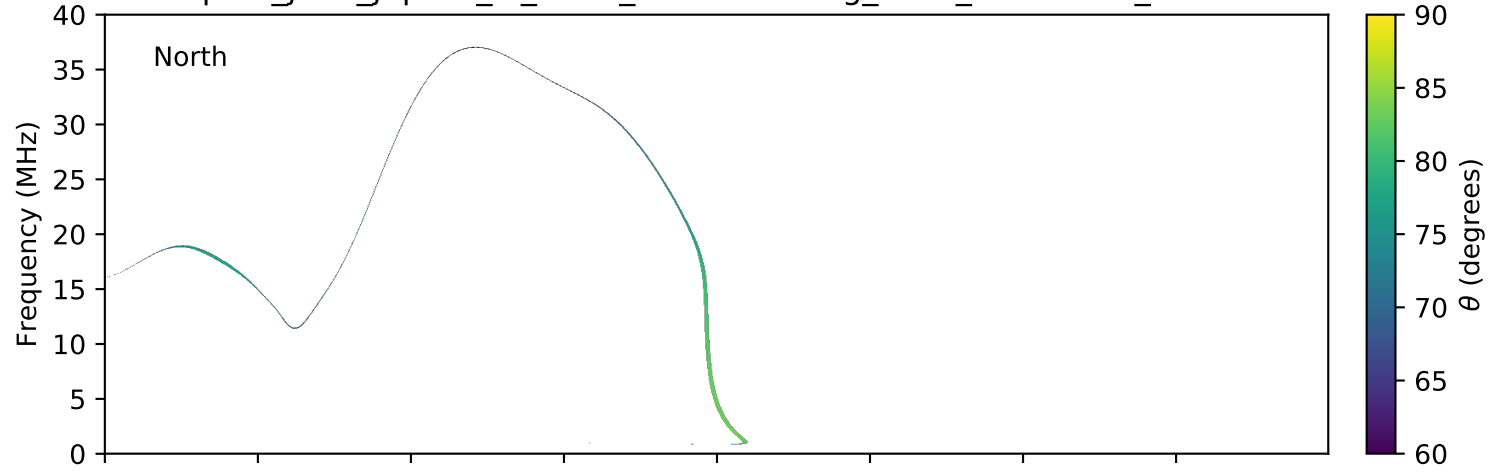
expres_juno_jupiter_io_isaac_lossc-wid1deg_3kev_20160911_v01.cdf
