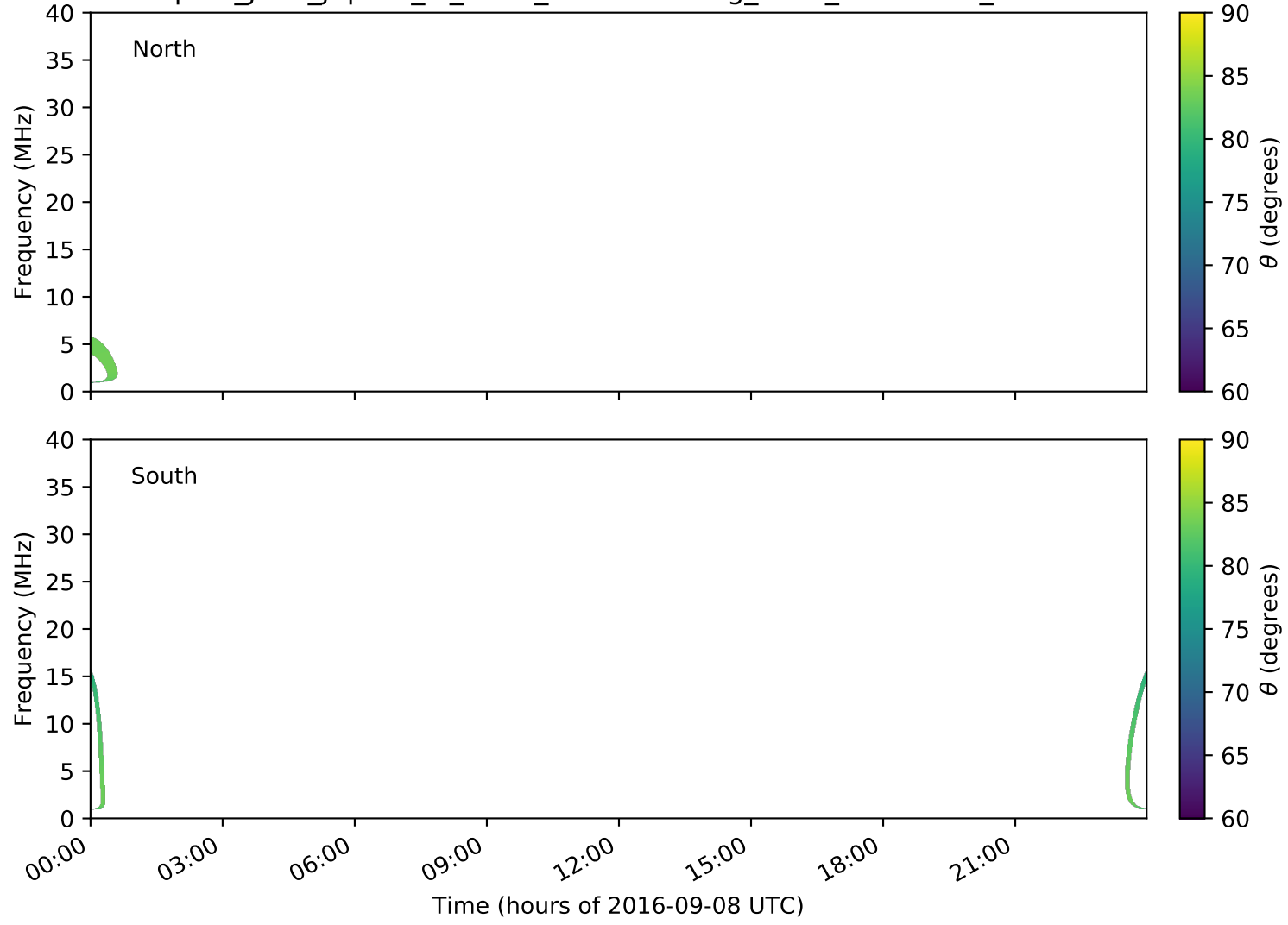
expres_juno_jupiter_io_isaac_lossc-wid1deg_3kev_20160908_v01.cdf
