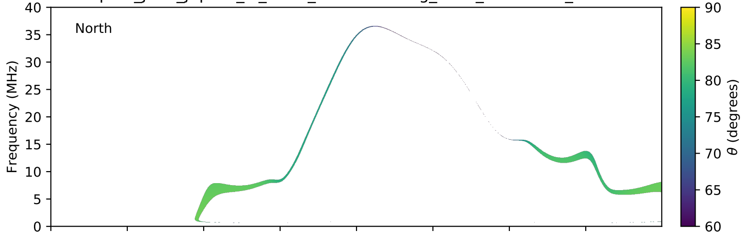
expres_juno_jupiter_io_isaac_lossc-wid1deg_3kev_20160907_v01.cdf
