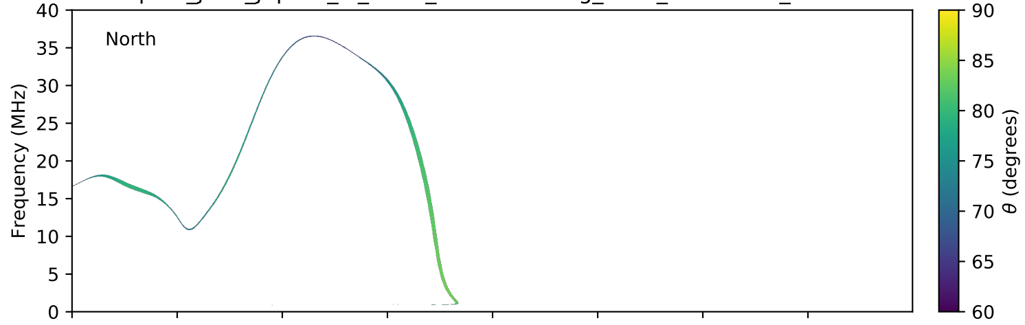
expres_juno_jupiter_io_isaac_lossc-wid1deg_3kev_20160904_v01.cdf
