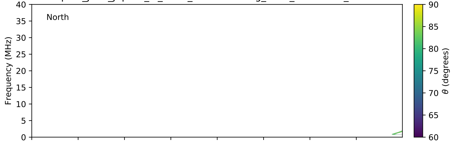
expres_juno_jupiter_io_isaac_lossc-wid1deg_3kev_20160901_v01.cdf
