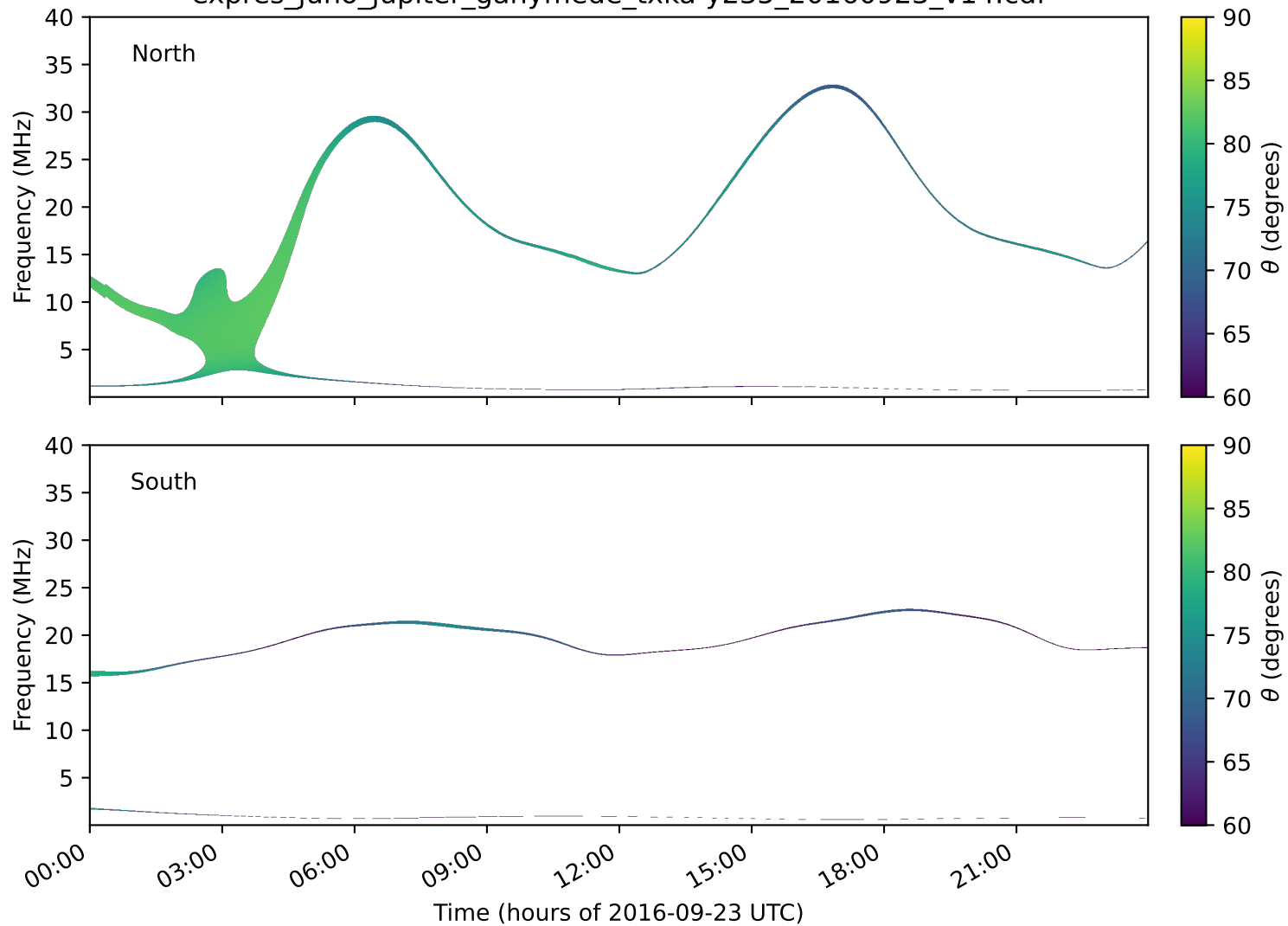
expres_juno_jupiter_ganymede_txka-y235_20160923_v14.cdf
