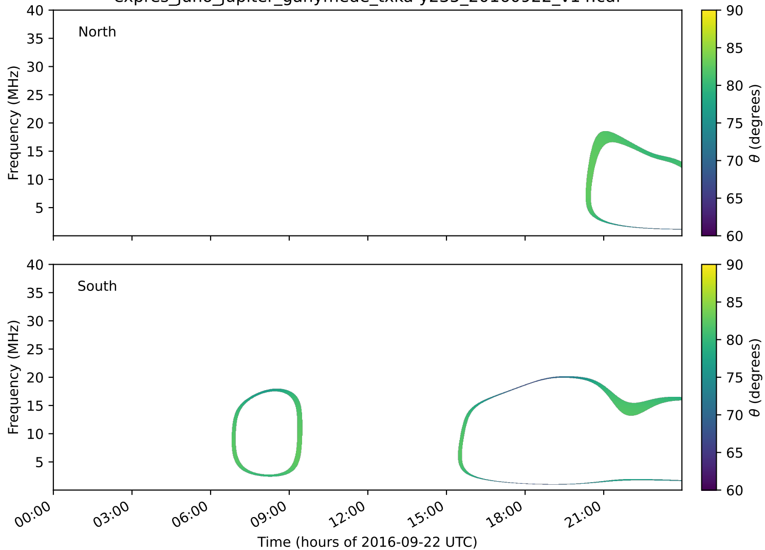
expres_juno_jupiter_ganymede_txka-y235_20160922_v14.cdf
