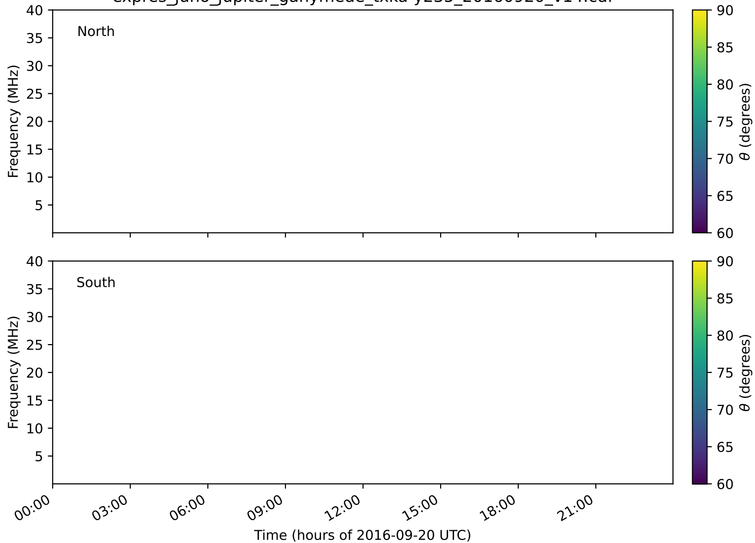
expres_juno_jupiter_ganymede_txka-y235_20160920_v14.cdf
