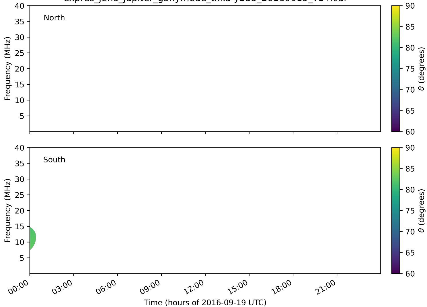
expres_juno_jupiter_ganymede_txka-y235_20160919_v14.cdf
