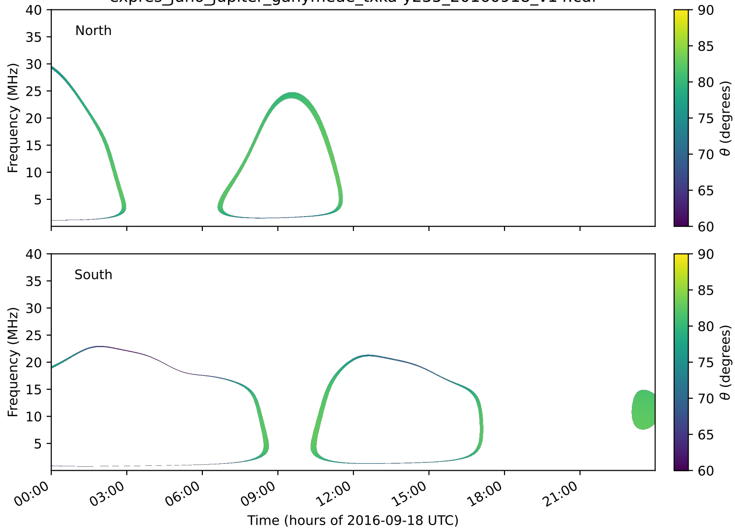
expres_juno_jupiter_ganymede_txka-y235_20160918_v14.cdf
