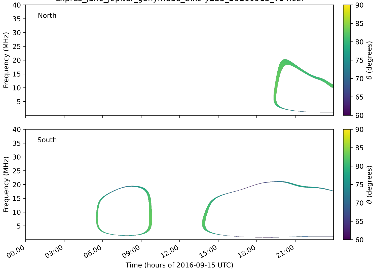
expres_juno_jupiter_ganymede_txka-y235_20160915_v14.cdf
