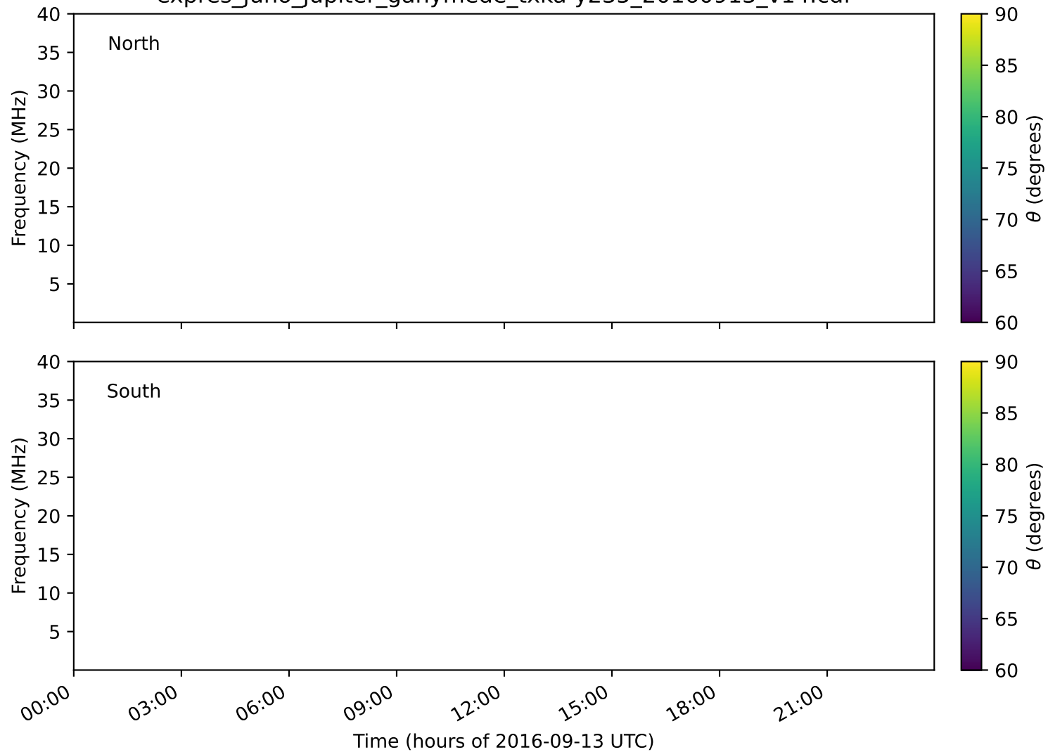
expres_juno_jupiter_ganymede_txka-y235_20160913_v14.cdf
