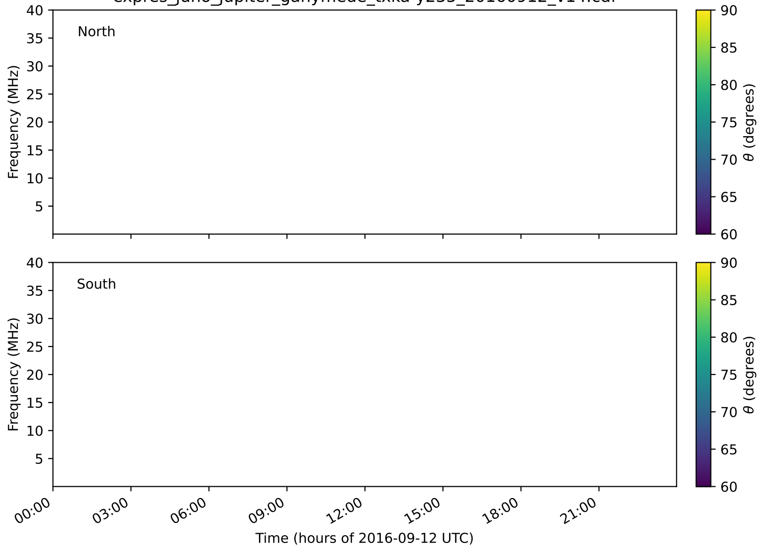
expres_juno_jupiter_ganymede_txka-y235_20160912_v14.cdf
