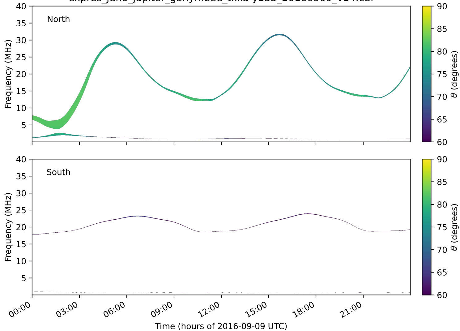
expres_juno_jupiter_ganymede_txka-y235_20160909_v14.cdf
