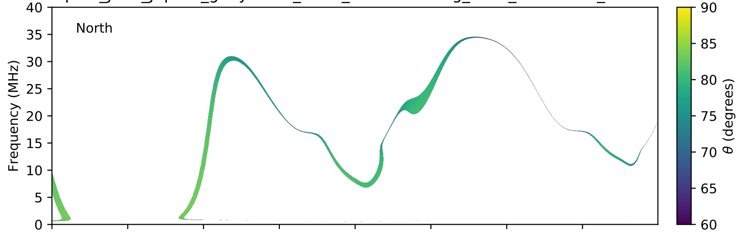
expres_juno_jupiter_ganymede_isaac_lossc-wid1deg_3kev_20160930_v01.cdf
