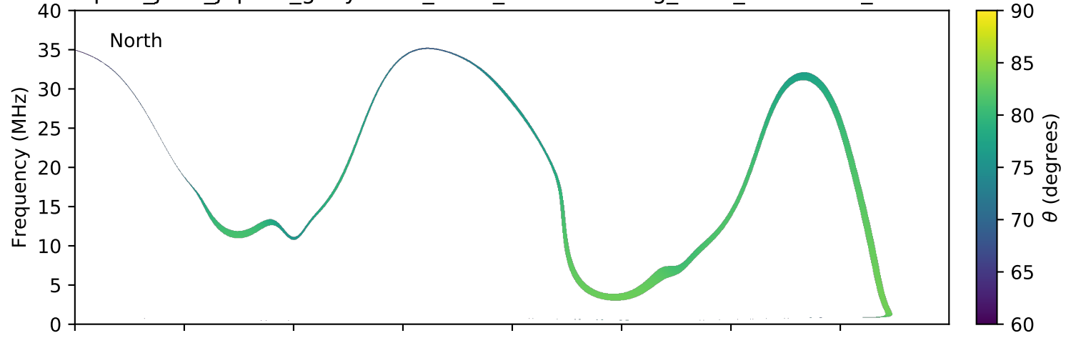
expres_juno_jupiter_ganymede_isaac_lossc-wid1deg_3kev_20160925_v01.cdf
