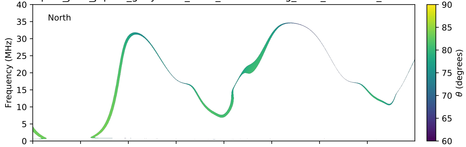
expres_juno_jupiter_ganymede_isaac_lossc-wid1deg_3kev_20160923_v01.cdf
