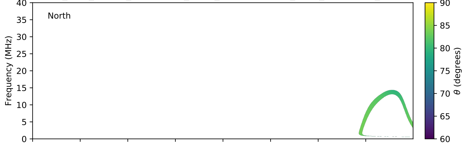
expres_juno_jupiter_ganymede_isaac_lossc-wid1deg_3kev_20160922_v01.cdf
