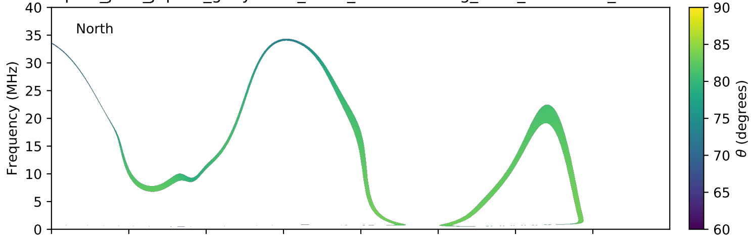
expres_juno_jupiter_ganymede_isaac_lossc-wid1deg_3kev_20160918_v01.cdf
