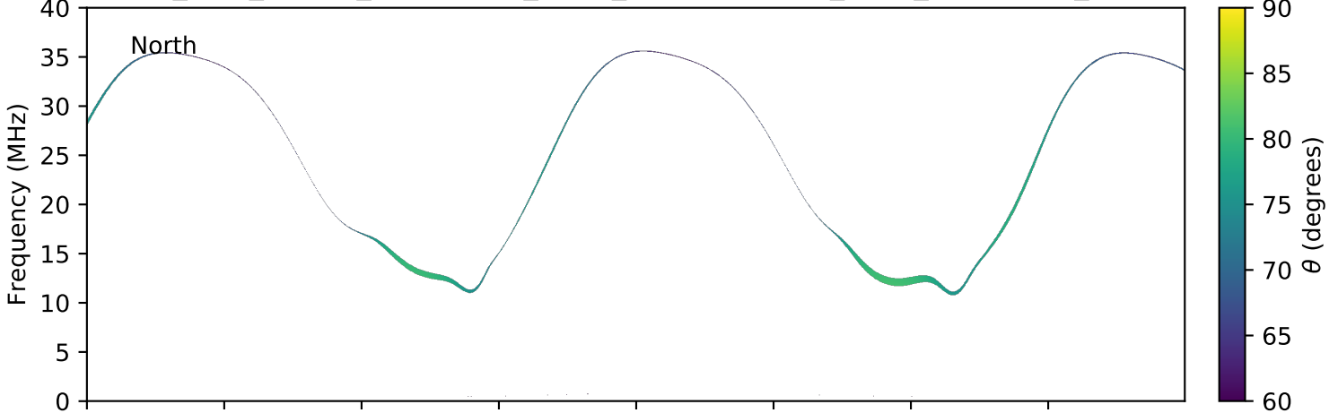
expres_juno_jupiter_ganymede_isaac_lossc-wid1deg_3kev_20160917_v01.cdf
