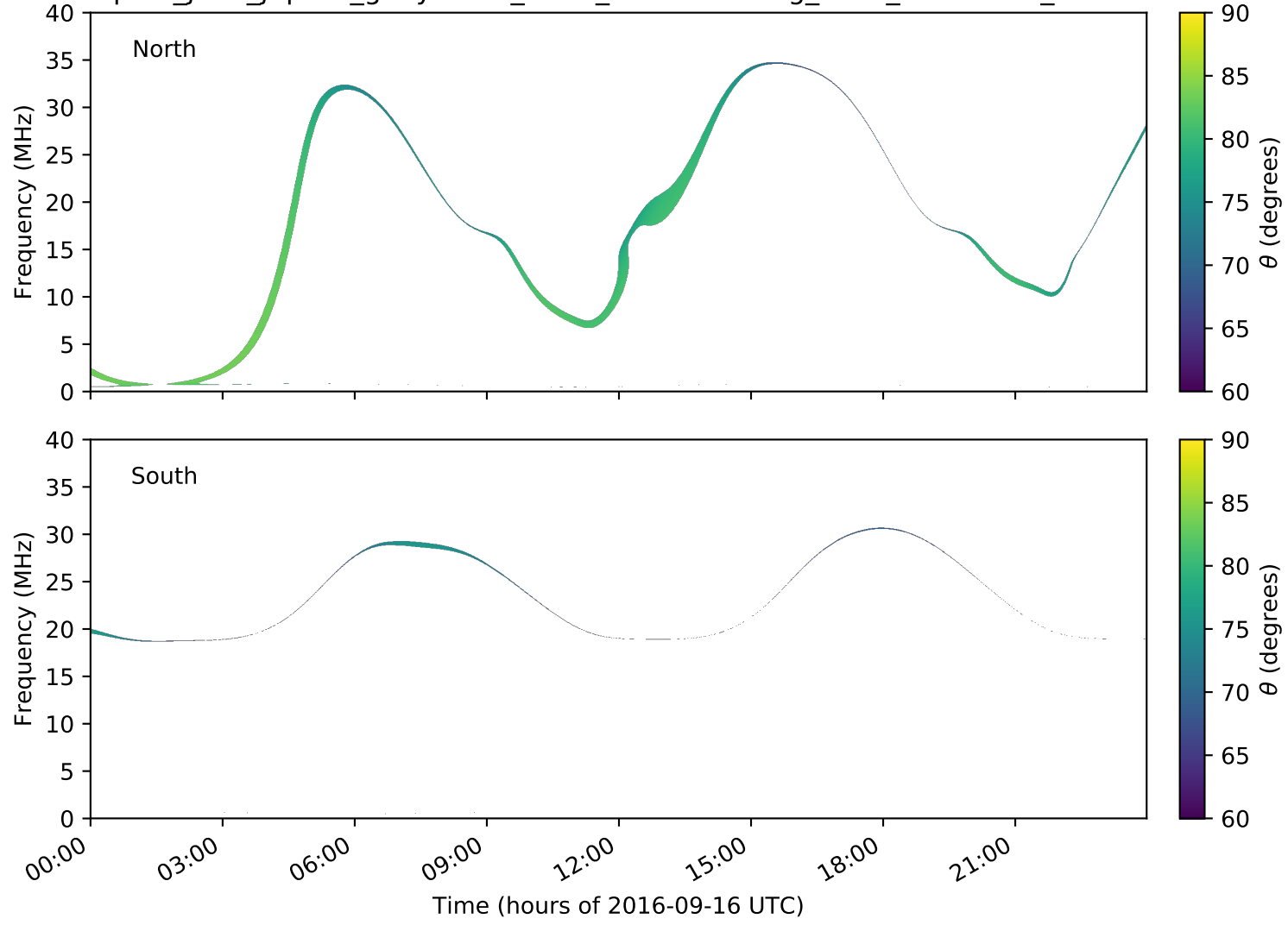
expres_juno_jupiter_ganymede_isaac_lossc-wid1deg_3kev_20160916_v01.cdf
