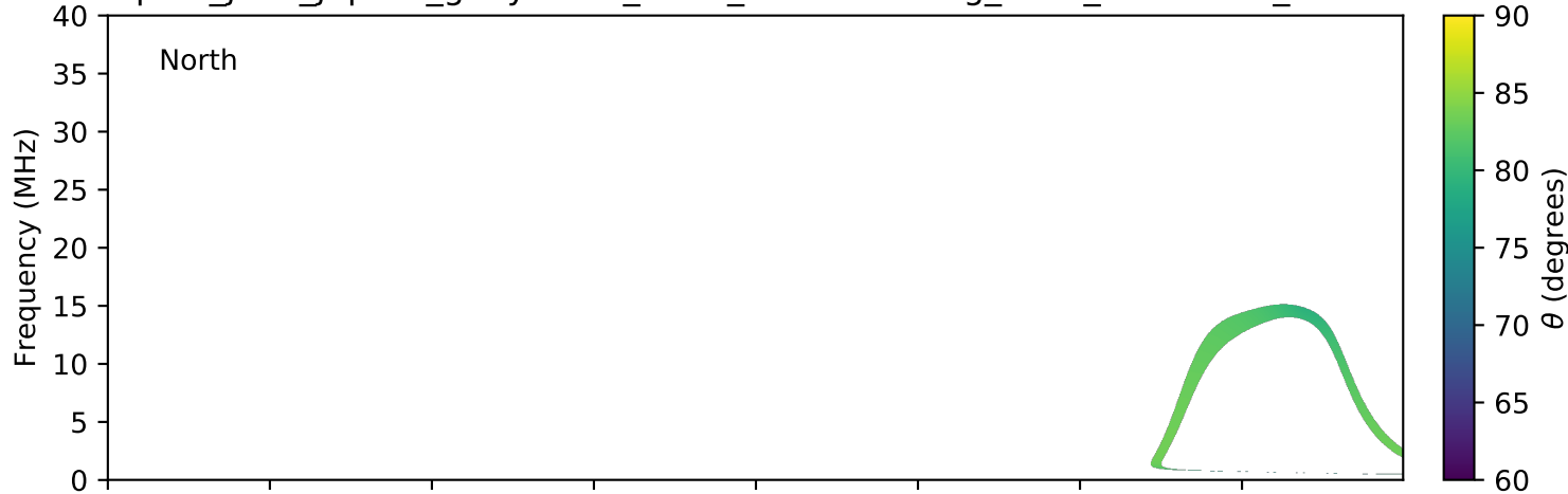
expres_juno_jupiter_ganymede_isaac_lossc-wid1deg_3kev_20160915_v01.cdf
