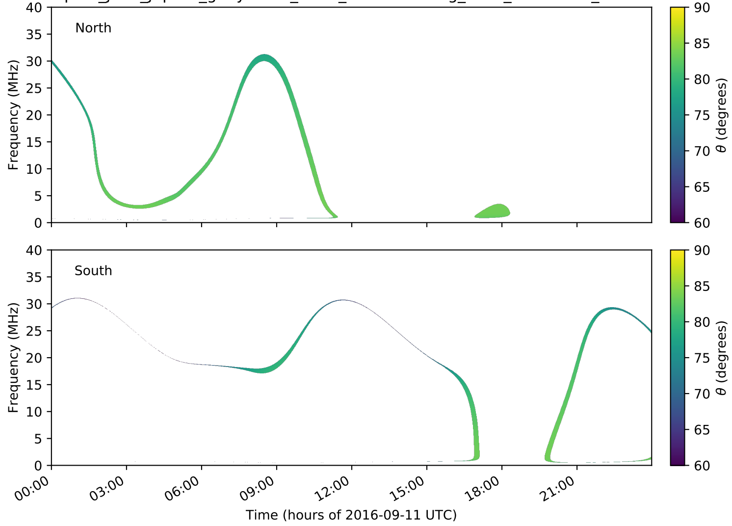
expres_juno_jupiter_ganymede_isaac_lossc-wid1deg_3kev_20160911_v01.cdf
