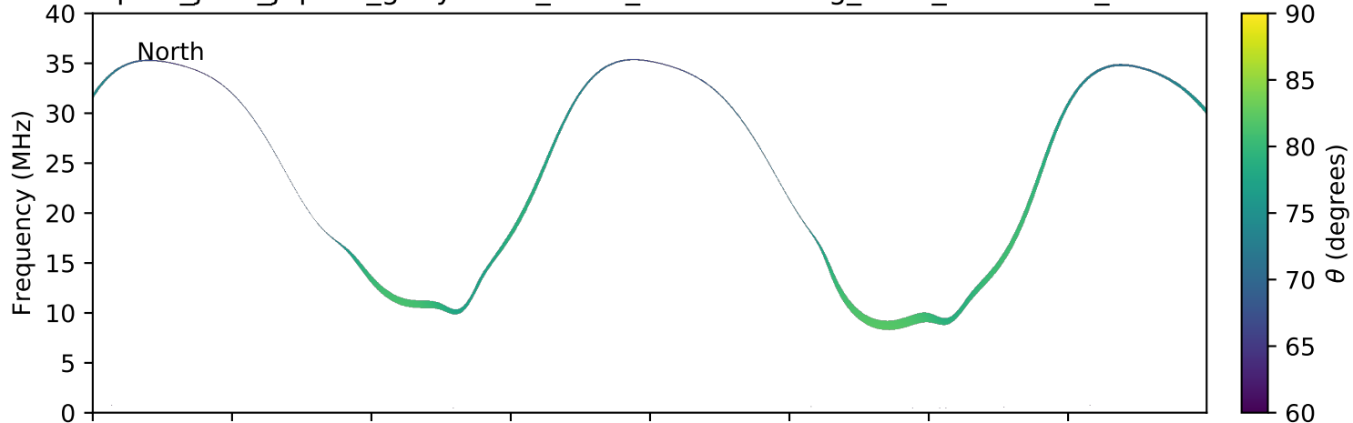
expres_juno_jupiter_ganymede_isaac_lossc-wid1deg_3kev_20160910_v01.cdf
