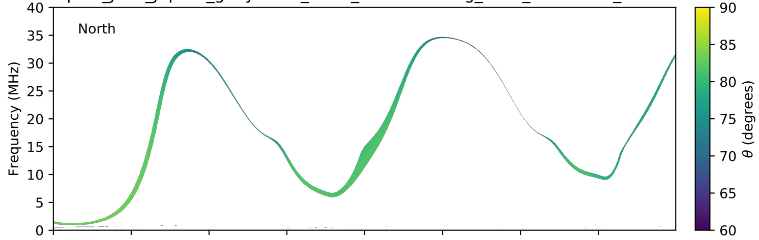
expres_juno_jupiter_ganymede_isaac_lossc-wid1deg_3kev_20160909_v01.cdf
