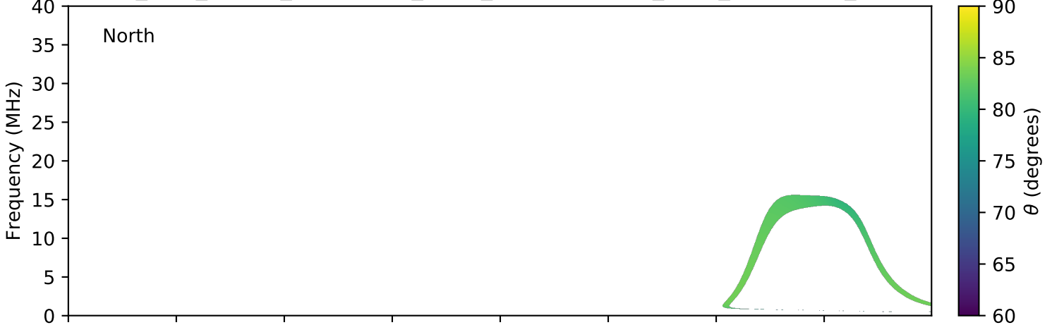
expres_juno_jupiter_ganymede_isaac_lossc-wid1deg_3kev_20160908_v01.cdf
