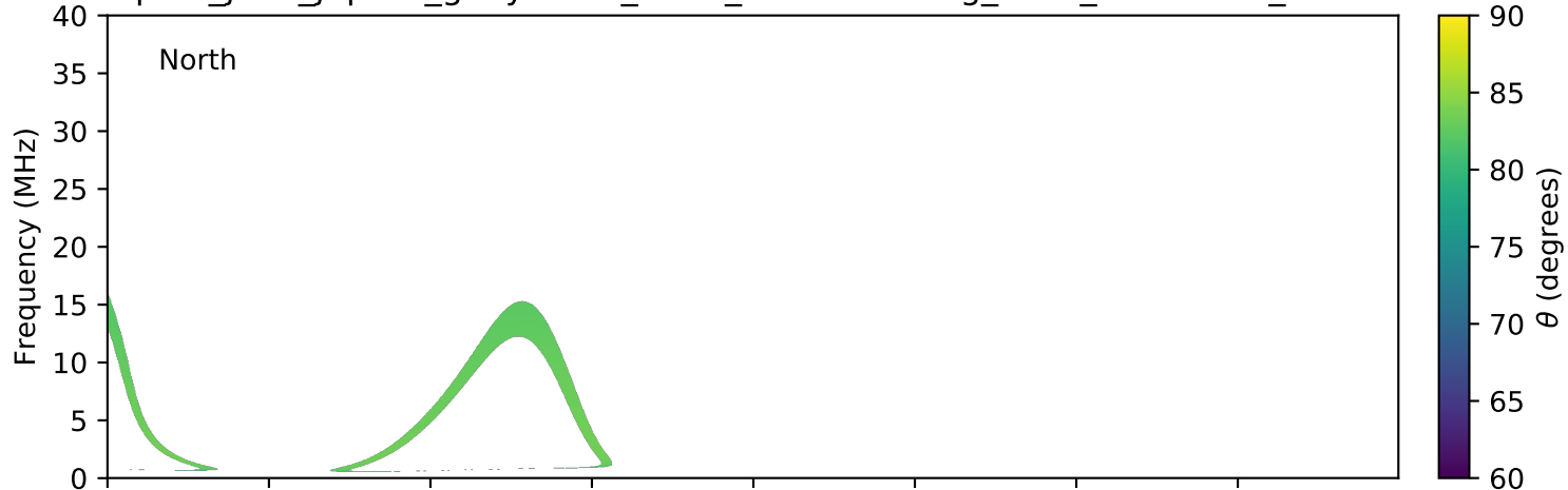
expres_juno_jupiter_ganymede_isaac_lossc-wid1deg_3kev_20160904_v01.cdf
