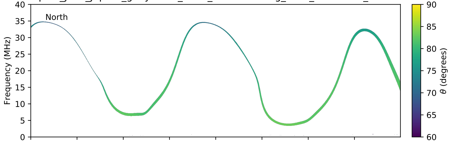
expres_juno_jupiter_ganymede_isaac_lossc-wid1deg_3kev_20160903_v01.cdf
