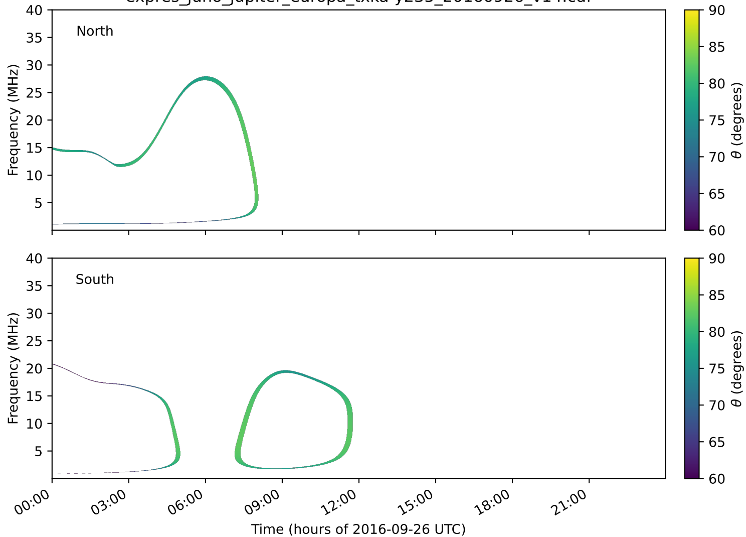
expres_juno_jupiter_europa_txka-y235_20160926_v14.cdf
