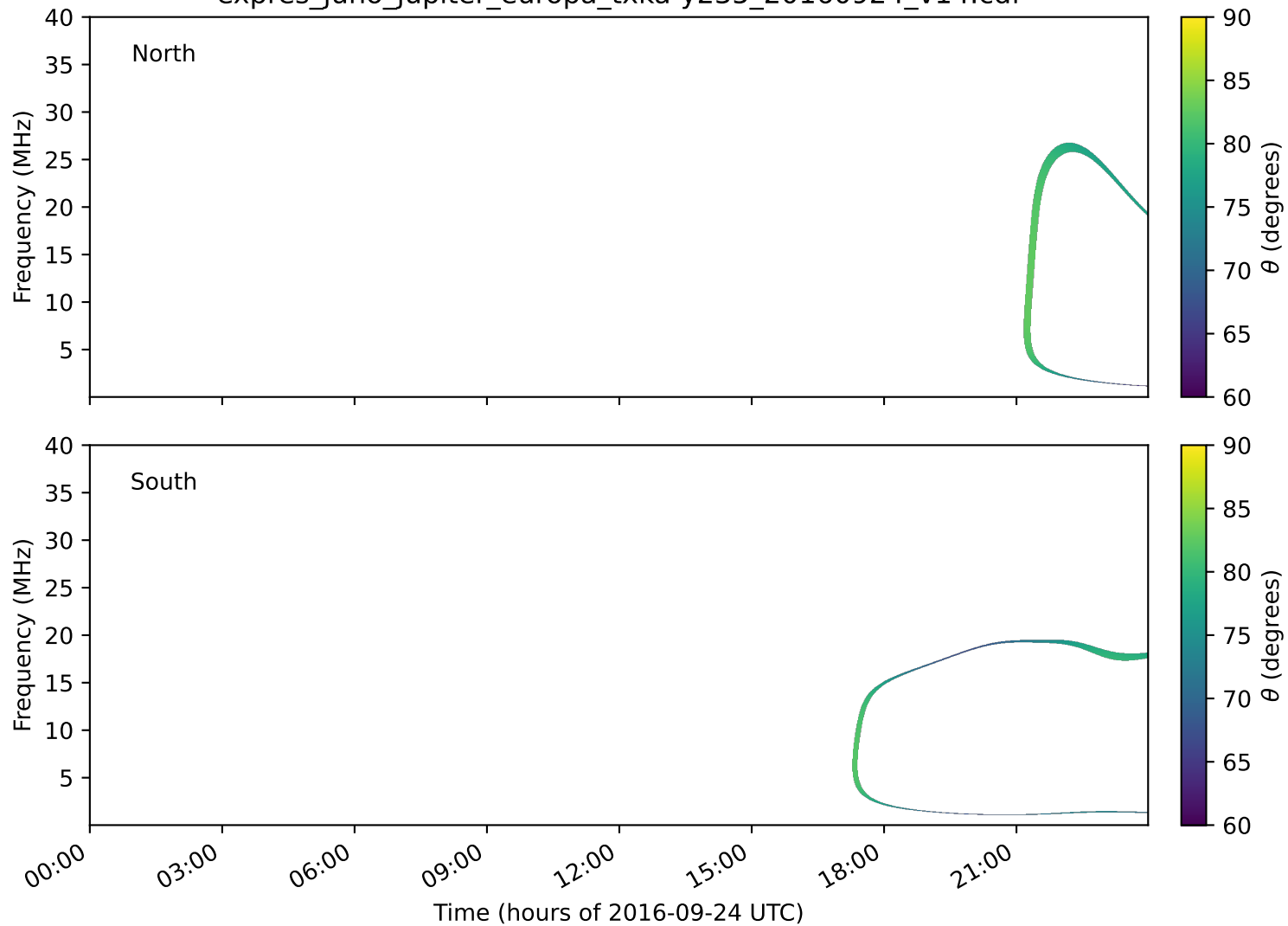
expres_juno_jupiter_europa_txka-y235_20160924_v14.cdf
