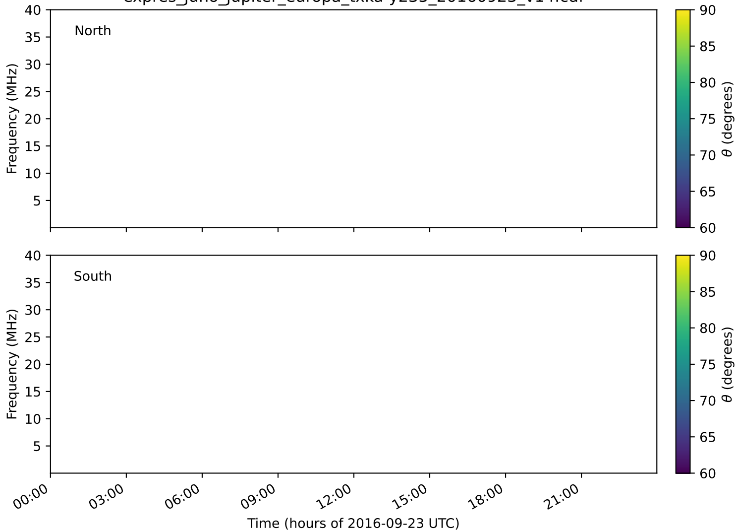
expres_juno_jupiter_europa_txka-y235_20160923_v14.cdf
