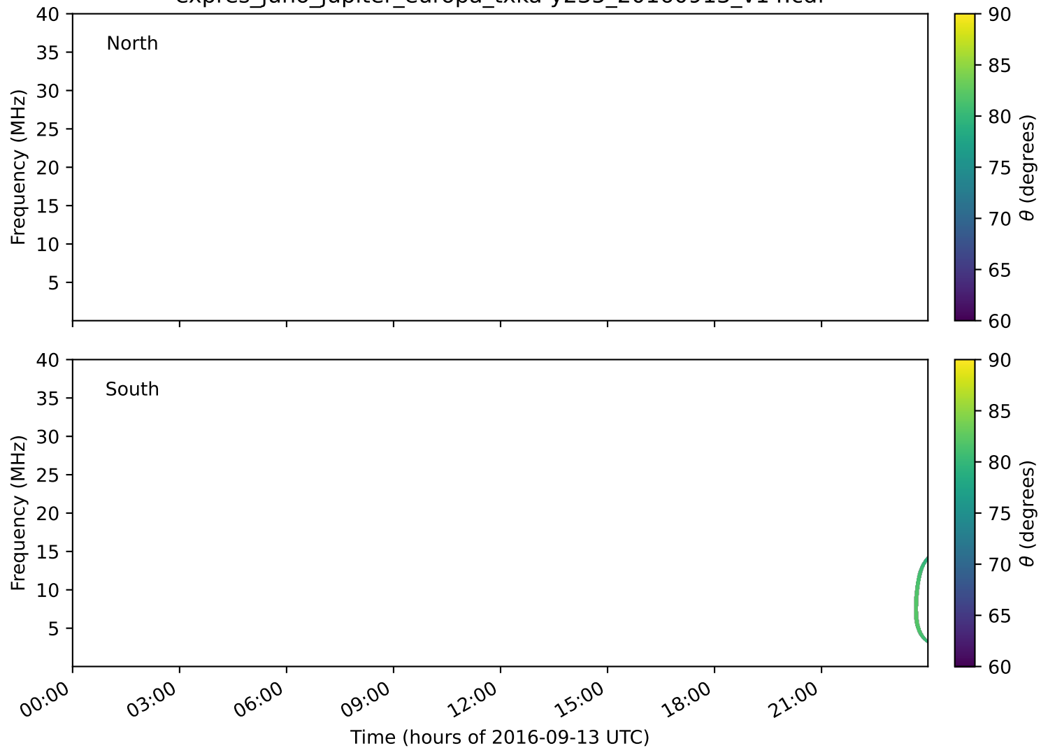
expres_juno_jupiter_europa_txka-y235_20160913_v14.cdf
