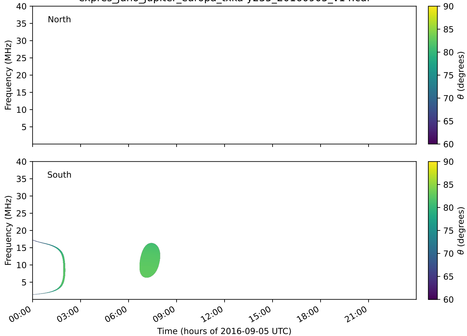
expres_juno_jupiter_europa_txka-y235_20160905_v14.cdf
