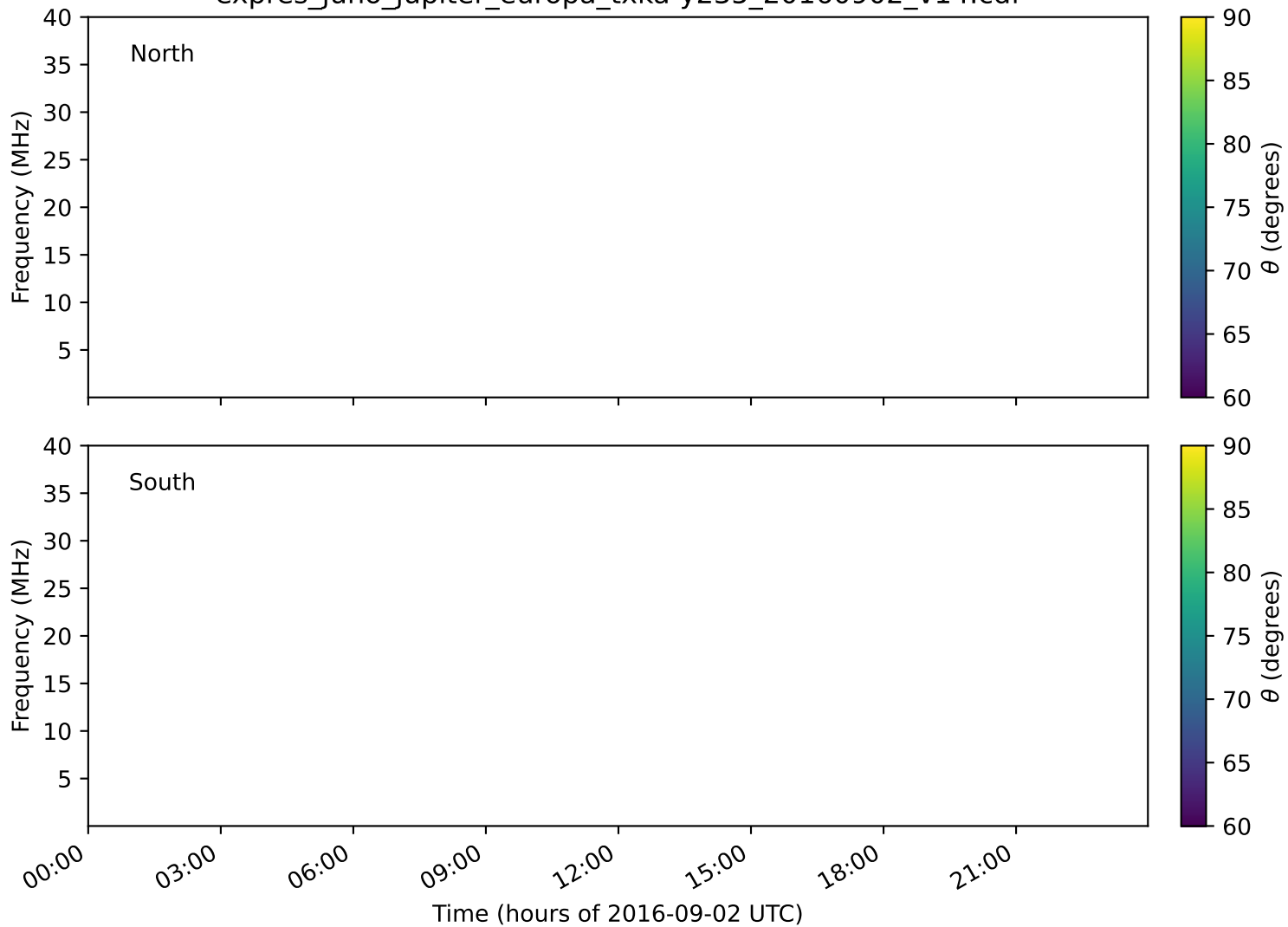
expres_juno_jupiter_europa_txka-y235_20160902_v14.cdf
