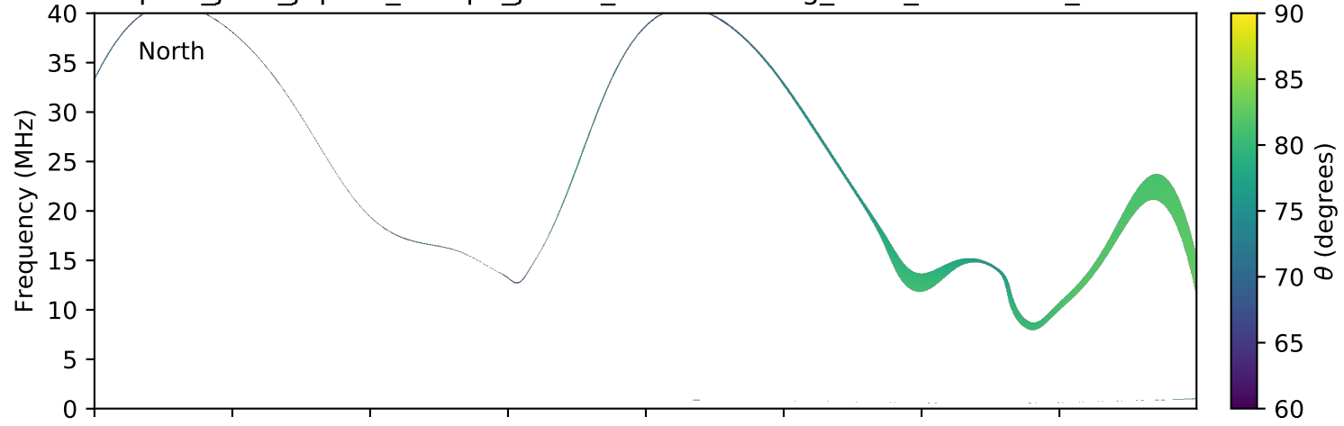
expres_juno_jupiter_europa_jrm09_lossc-wid1deg_3kev_20160929_v01.cdf
