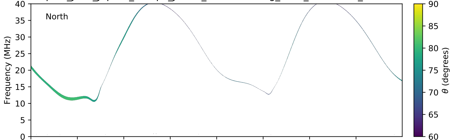
expres_juno_jupiter_europa_jrm09_lossc-wid1deg_3kev_20160925_v01.cdf
