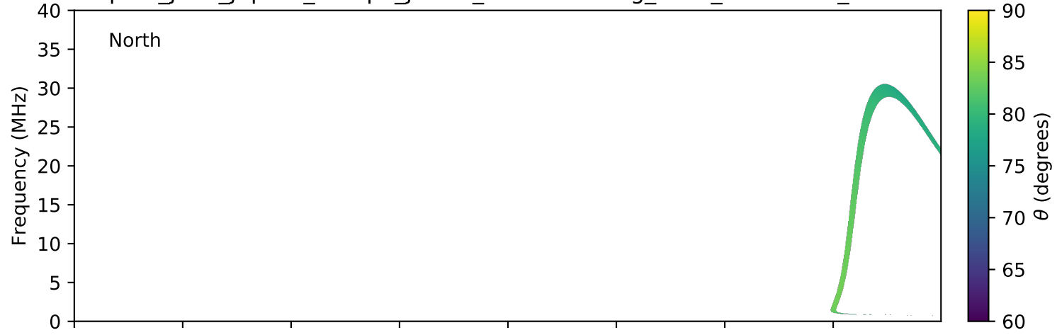
expres_juno_jupiter_europa_jrm09_lossc-wid1deg_3kev_20160924_v01.cdf
