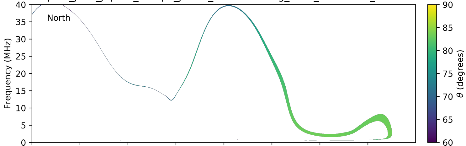
expres_juno_jupiter_europa_jrm09_lossc-wid1deg_3kev_20160922_v01.cdf
